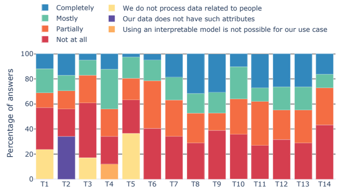
Fig. 2: Adoption of SE practices for trustworthy ML.
