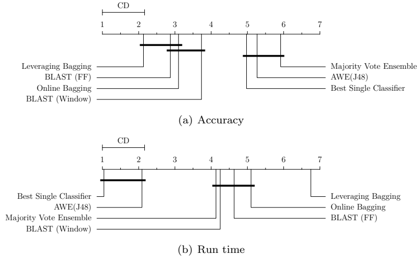
Fig. 11 Results of Nemenyi test, \alpha = 0.05 . Classifiers are sorted by their average rank (lower is better). Classifiers that are connected by a horizontal line are statistically equivalent.
