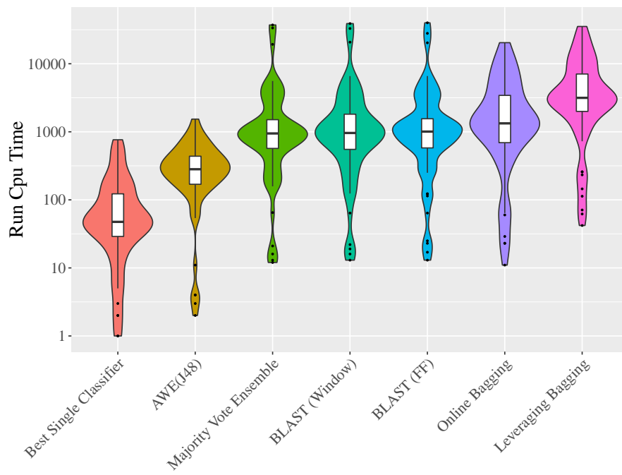
(b) Run time (in seconds)
