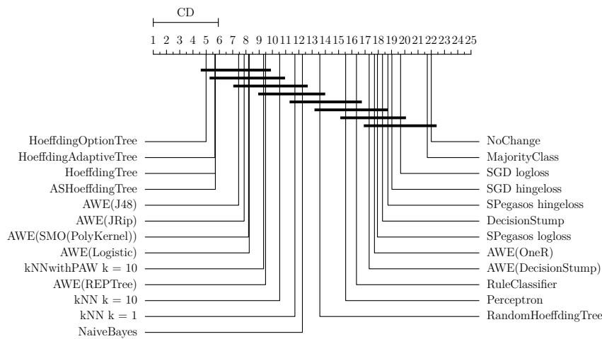
Fig. 6 Results of Nemenyi test ( \alpha = 0.05 ) on the predictive accuracy of the base-classifiers in this study.
