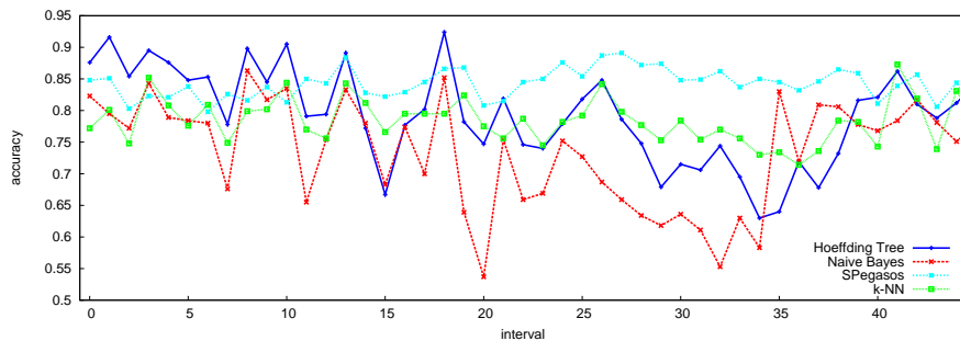
Fig. 1 Performance of four classifiers on intervals (size 1,000) of the electricity dataset. Each data point represents the accuracy of a classifier on the most recent interval.
