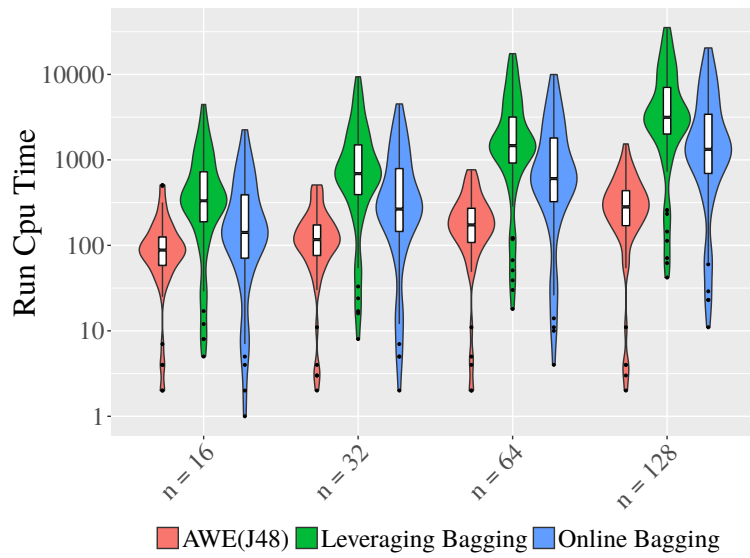
(b) Run time (in seconds)
