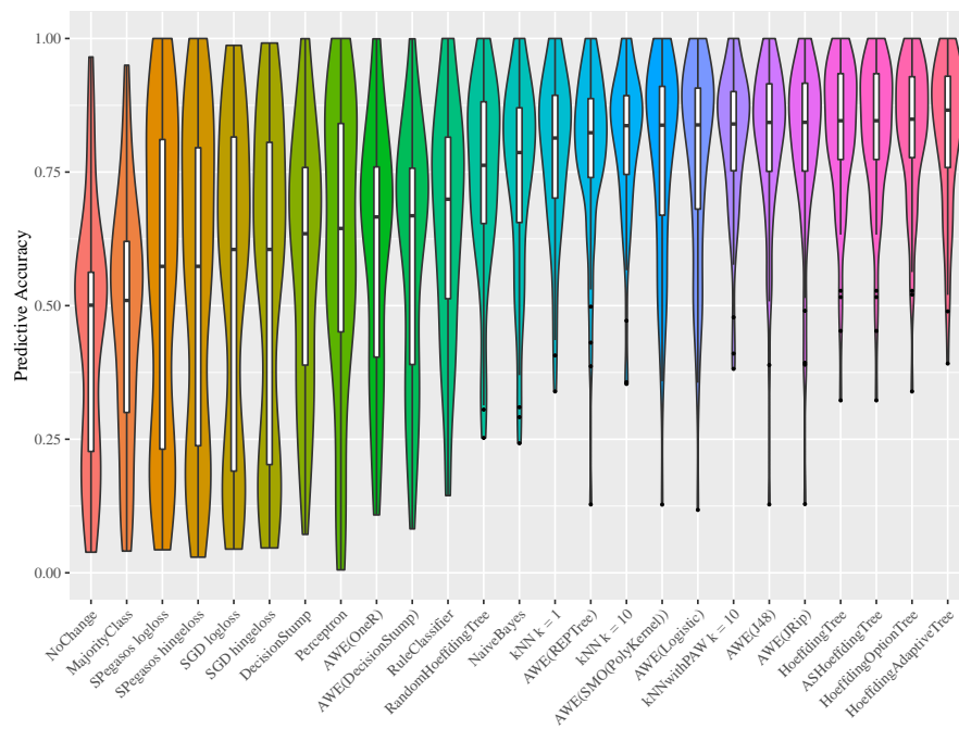
(a) Predictive Accuracy
