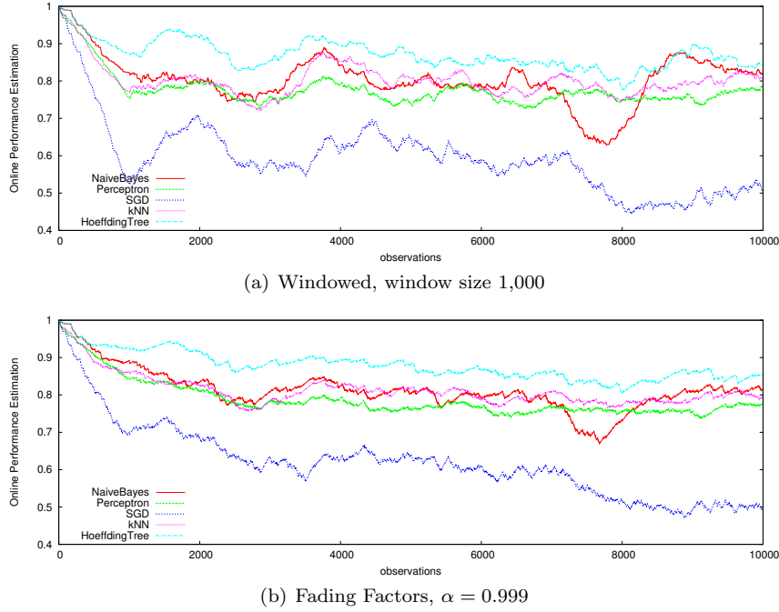
Fig. 4 Online performance estimation, i.e. the estimated performance of each algorithm given previous examples, measured on the start of the electricity data stream.
