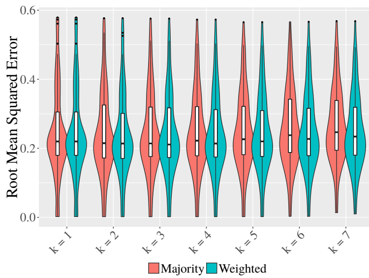
(b) Root Mean Squared Error
