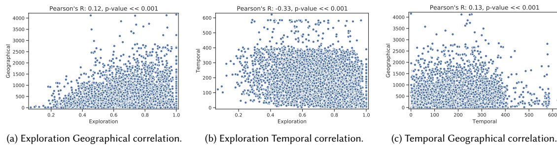
Fig. 4. User Behavior Aspects Correlation
