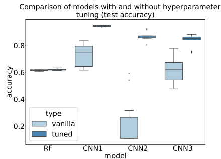
Fig. 1: Preliminary experiments using the EuroSAT dataset [9]. A random forest and three different CNNs built from scratch based on machine learning (a simple CNN with 3 convolutional layers (CNN1)) and remote sensing literature (CNN2 [1], CNN3 [15]) are compared. For each model, two versions are shown: a vanilla model performance using default configurations and a tuned model. The tuned models show the performance after applying hyperparameter tuning for the optimizer, learning rate, batch size, and the number of epochs in the case of the CNNs and the number of features for the random forest.
