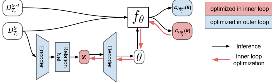
Fig. 27 Workflow of LEO. adapted from Rusu et al. (2018).
