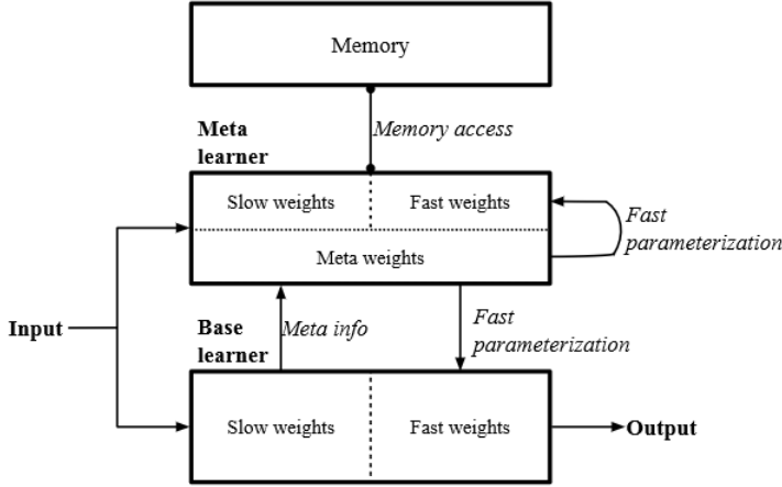
Fig. 15 Architecture of a Meta Network. Source: Munkhdalai and Yu (2017).
