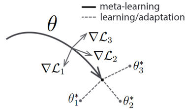
Fig. 24 MAML learns an initialization point from which it can perform well on various tasks. Source: Finn et al. (2017).
